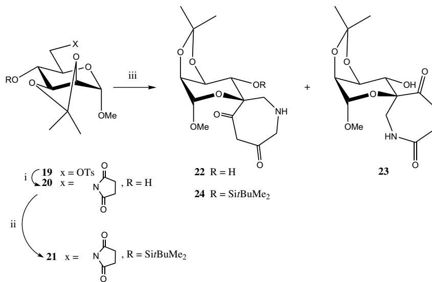
Scheme 2. Reagents and condition: (i) K succinimide, DMF; (ii) TFOSi i BuMe 2 , Py; (iii) 254 nm, CH 3 CN.
